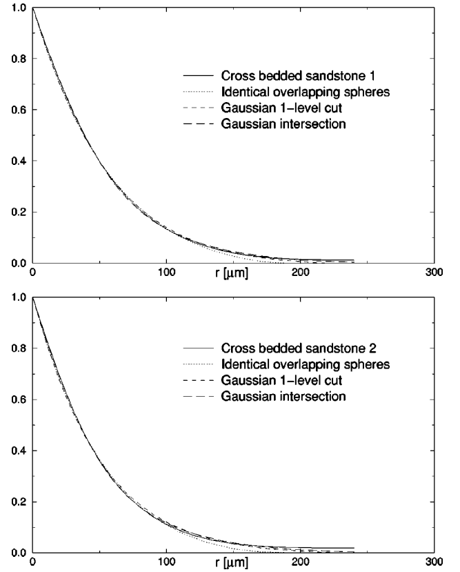
FIG. 18. Normalized two-point correlation functions S(r) of the two 300^3 sandstone samples and the averaged best fits for the model structures.
